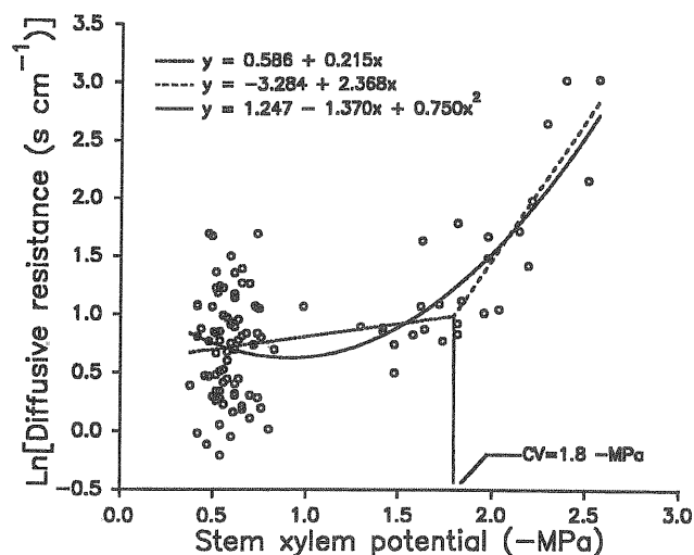
Fig 1. Relationship between Ilex cornuta 'Burfordii Nana' diffusive resistance and xylem potential during 8 days without irrigation.
