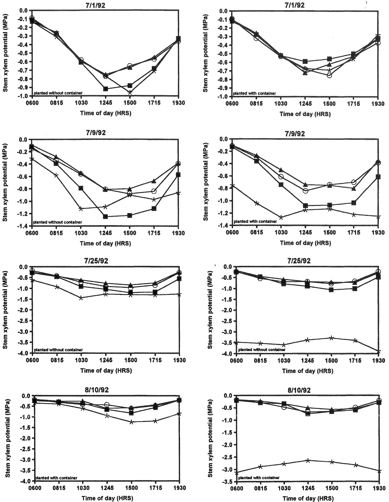
Fig 2. Ilex cornuta 'Burfordii Nana' Diurnal xylem potential in each irrigation treatment after transplanting to simulated landscape and with or without container removed from root ball. Plants were irrigated every day (triangle), every two days (circle), every four days (square) or every 14-16 days (star).
